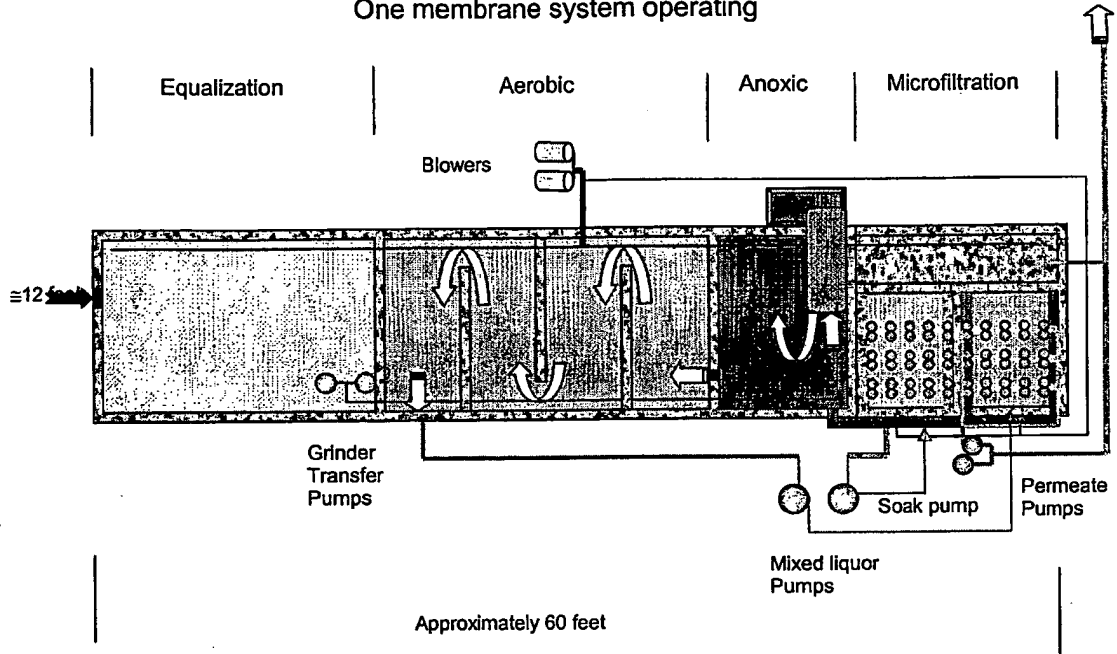
Figure 18 - Soak Phase One membrane system operating
